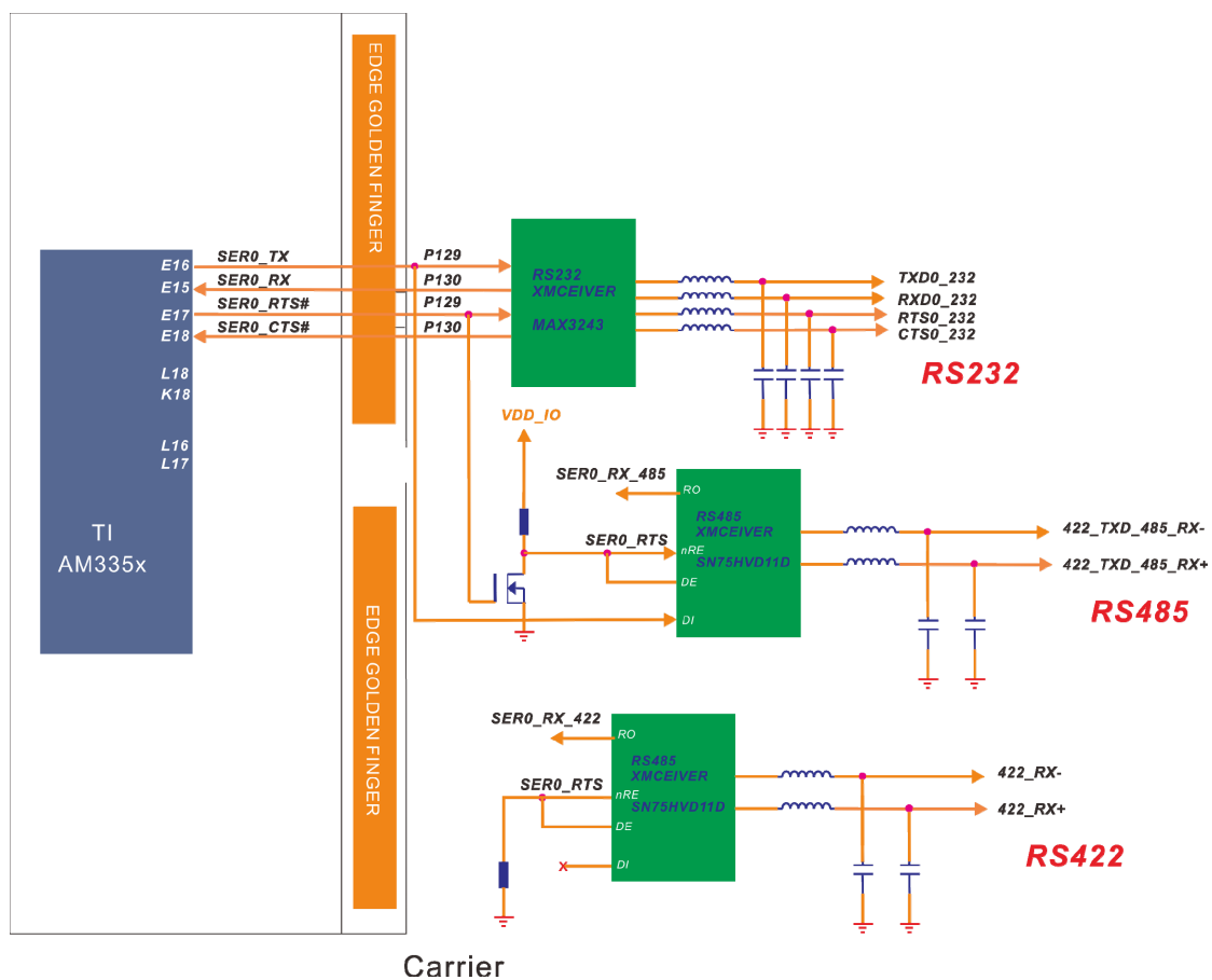
Figure 28: RS232, RS422 and RS485 System Block Diagram
