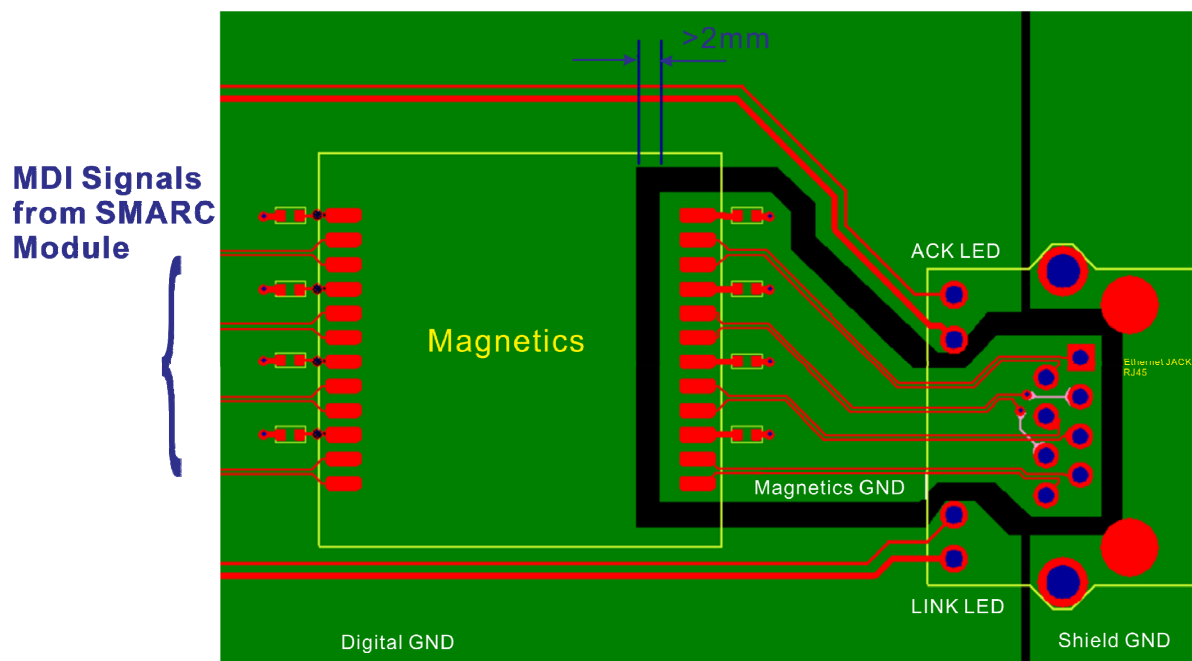
Figure 9: Separation of Magnetics Ground
