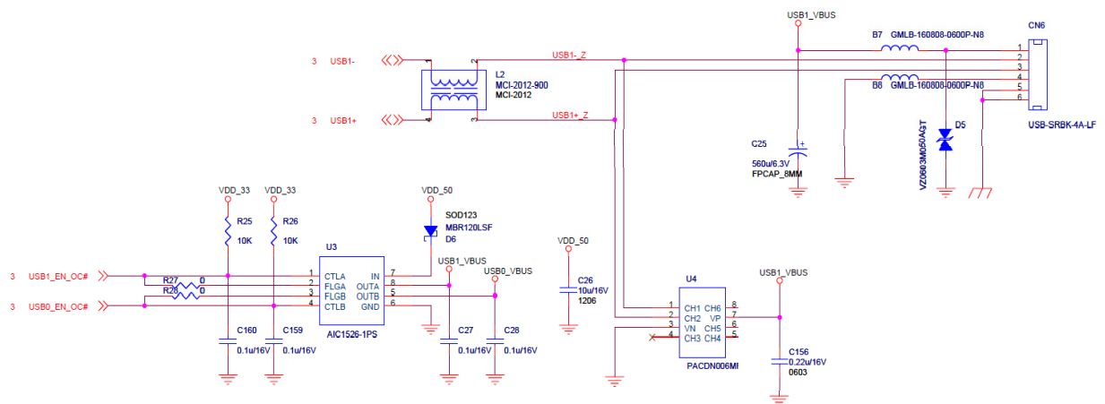
Figure 15: USB Host Reference Schematic
