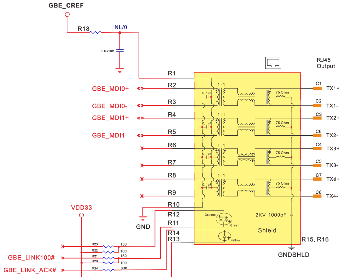
Figure 11: Fast Ethernet with Integrated Magnetics Reference Schematic
