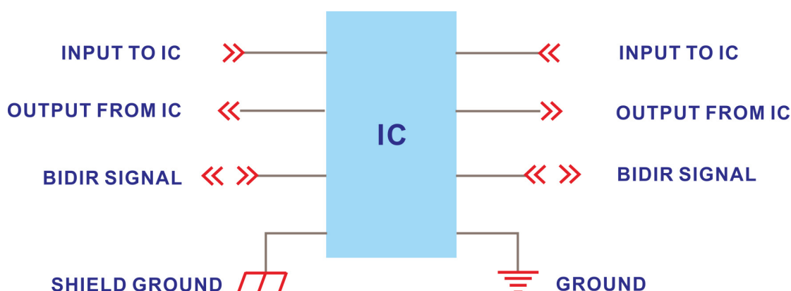
Figure 1: Schematic Conventions
