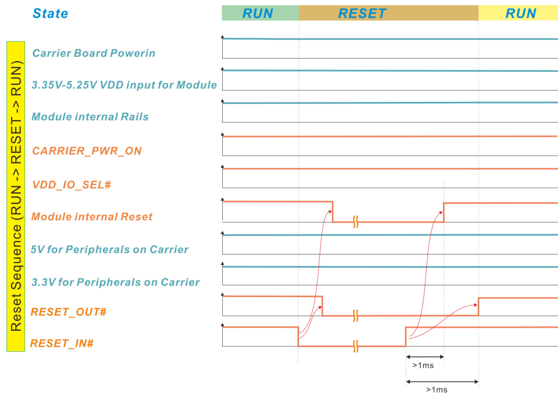
Figure 41: Reset Sequence
