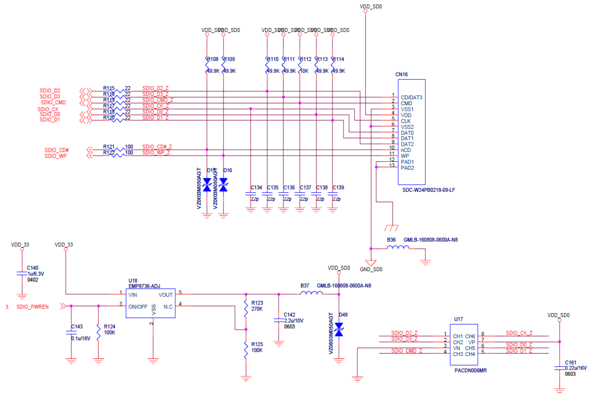
Figure 23: SD/SDHC Interface Reference Schematic
