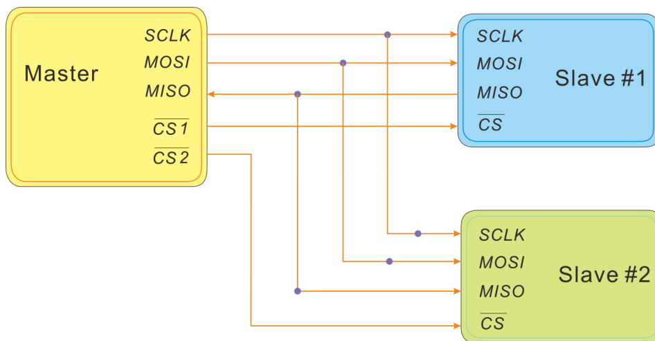
Figure 31: SPI with Multi-Slave Configuration
