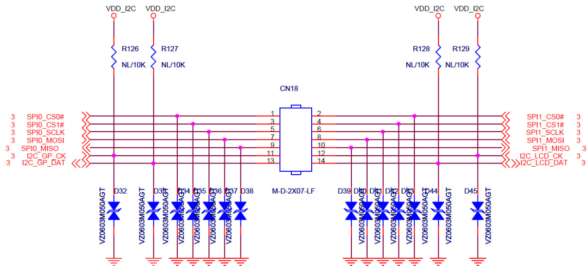
Figure 32: SPI Signals Reference Schematic
