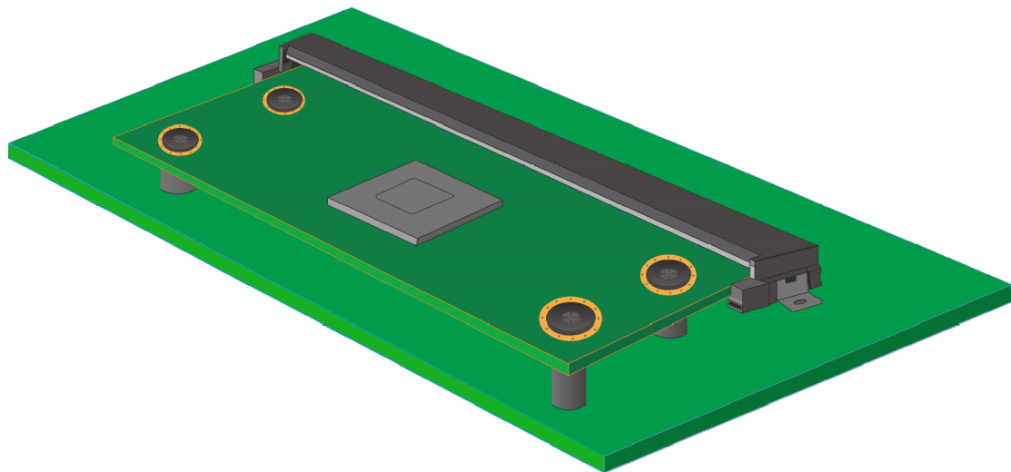
Figure 48: Screw Fixation
