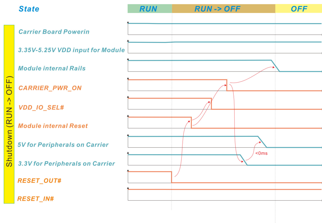
Figure 40: Shutdown Sequence
