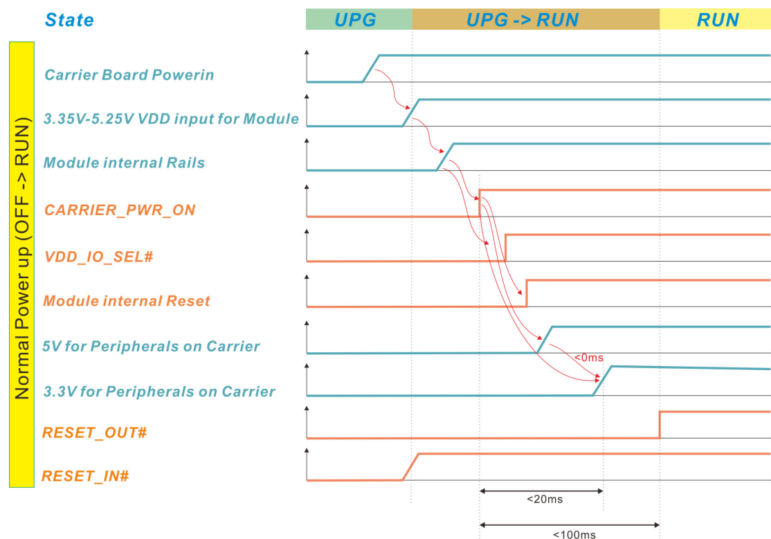
Figure 39: Power-Up Sequence
