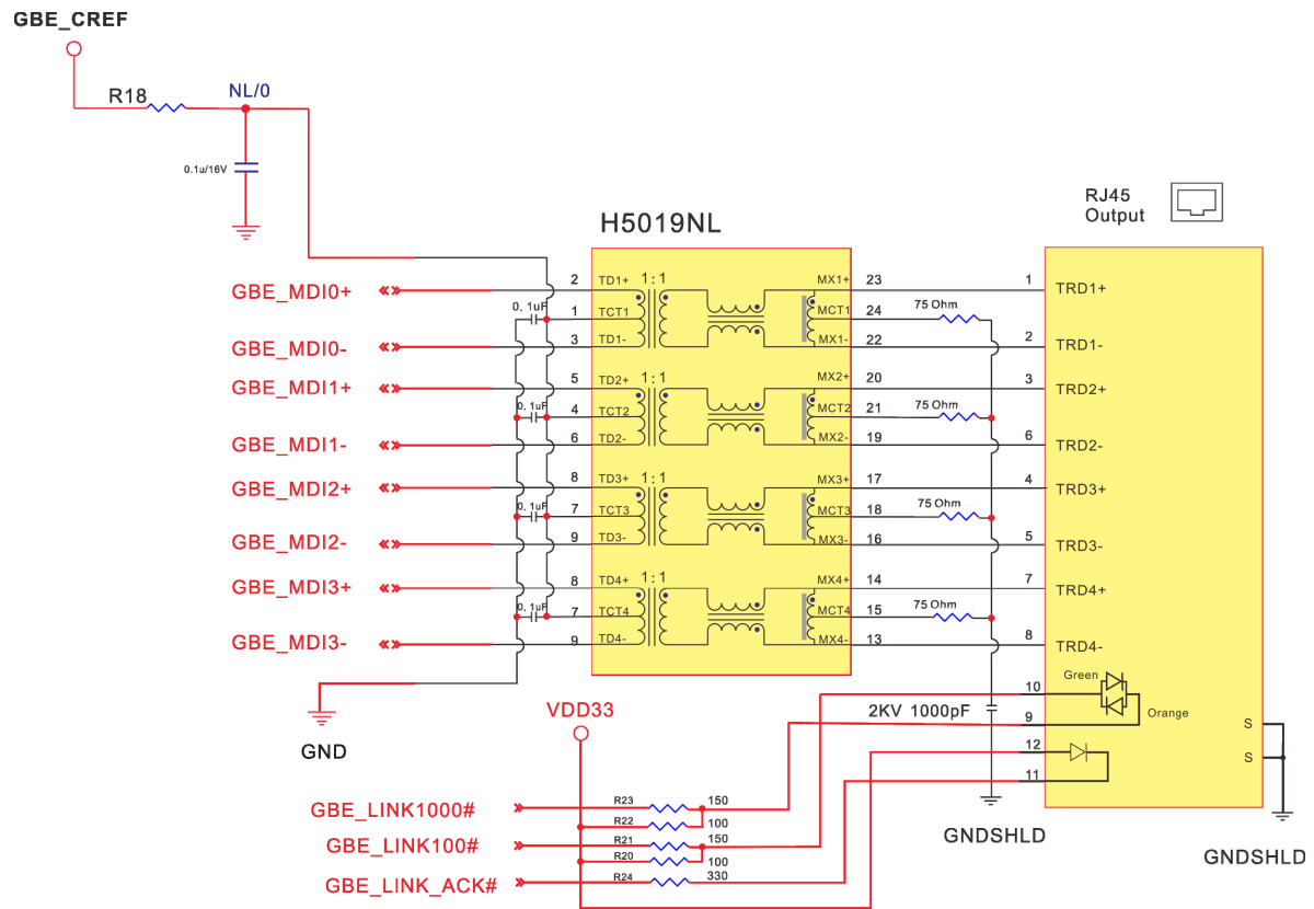
Figure 10: Gigabit Ethernet with Discrete Magnetics Reference Schematic
