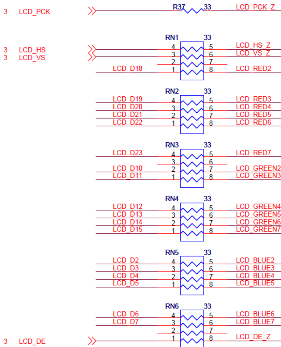
Figure 17: LCD Data Line with Serial Resistors
