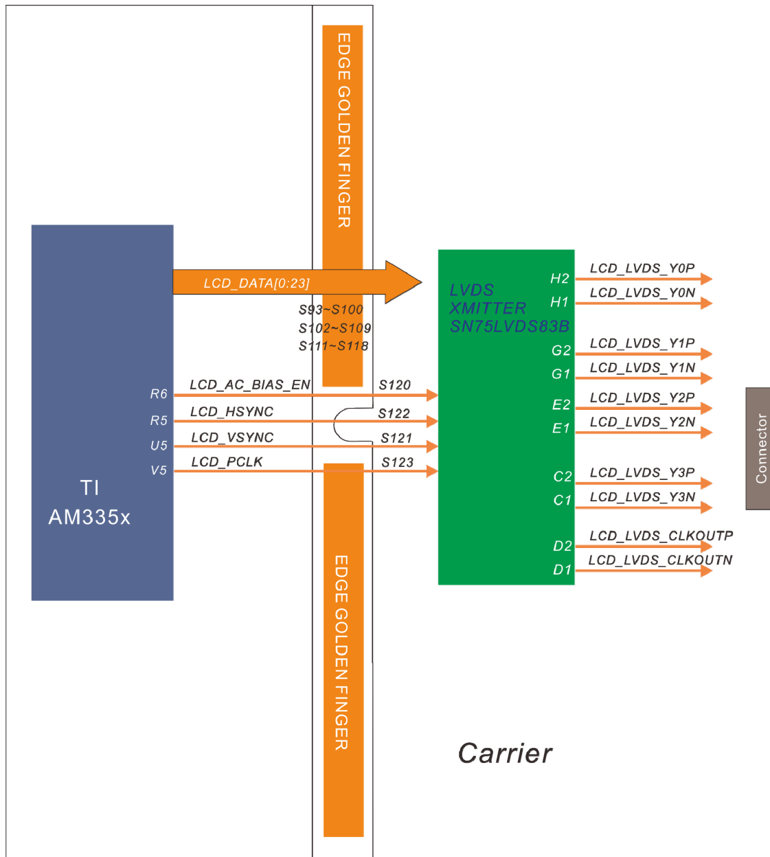
Figure 21: Carrier Based 24-bit LVDS Connection
