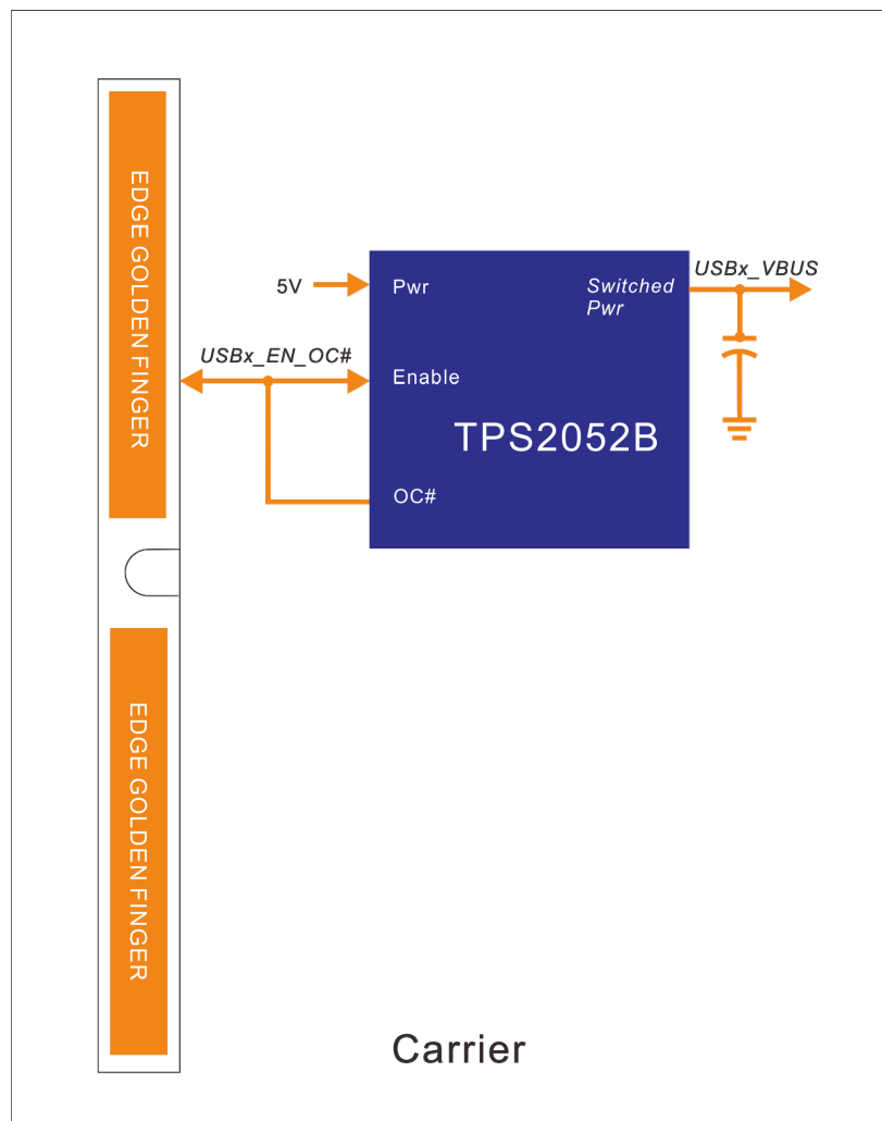
Figure 12: USB_EN_OC# and USB Power Switch Block Diagram
