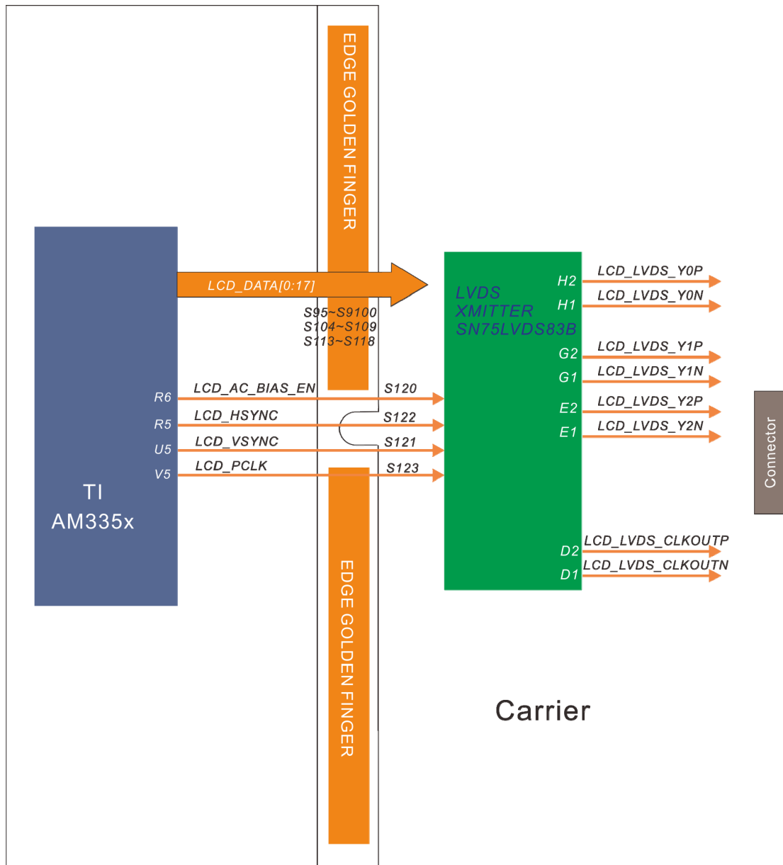
Figure 20: Carrier Based 18-bit LVDS Connection
